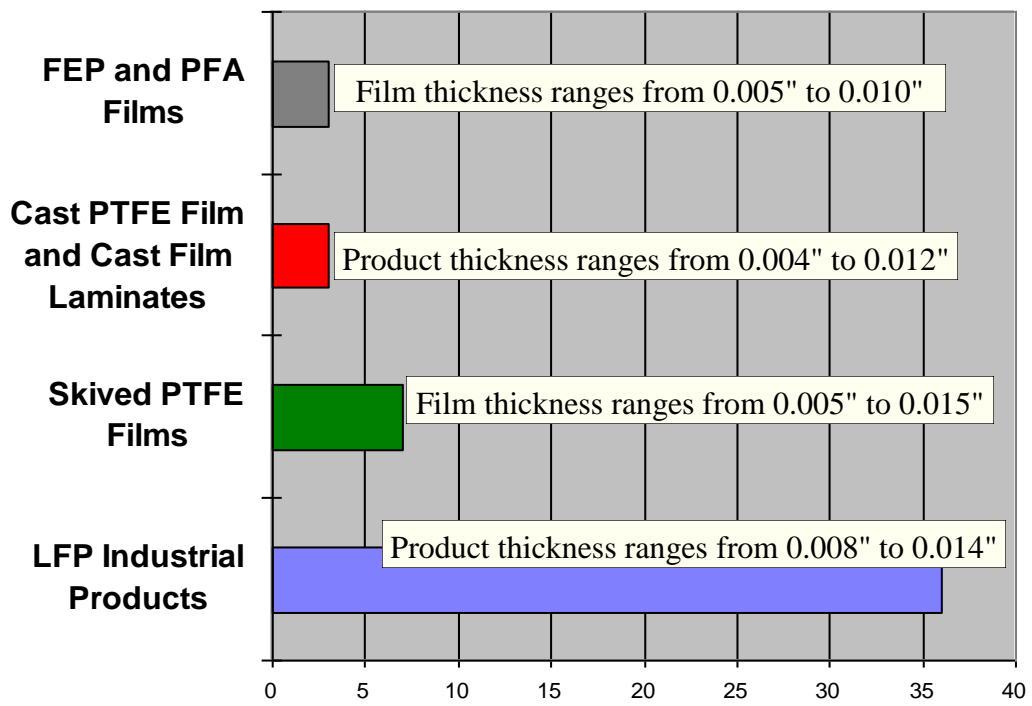
Hours to Failure in Flex Tester (30,600 cycles/hour)
