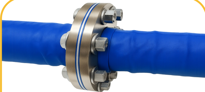
Factory-Installed Bolt Flange, Connected to Matching Factory-Installed Bolt Flange.
